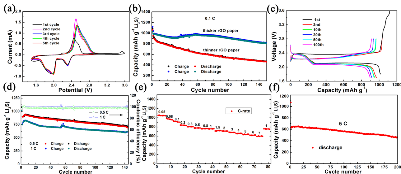
Figure 5. (a) Cyclic voltammograms of the nano- \text{Li}_2\text{S} /rGO paper electrode between 1.5 and 3.6 V at the first cycle and the following four cycles scan between 1.5 and 3 V at a potential scanning rate of 0.2 \text{ mV s}^{-1} . Electrochemical characteristics of the nano- \text{Li}_2\text{S} /rGO paper electrodes. All electrodes were charged to 3.6 V at the first cycle in 0.05 C rate and then cycled between 1.7–2.8 V. Electrolyte was 0.6 M LiTFSI with the additive of 0.01 M \text{Li}_2\text{S} and 0.4 M \text{LiNO}_3 . (b) Cycling performance of the thicker and thinner nano- \text{Li}_2\text{S} /rGO papers at a current rate of 0.1 C. (c) Charge and discharge profiles of the thicker nano- \text{Li}_2\text{S} /rGO paper at the 1st, 2nd, 10th, 20th, 50th, 100th cycle at 0.1 C. (d) Cycling performance and corresponding Coulombic efficiency at current rates of 0.5 and 1 C for the thicker nano- \text{Li}_2\text{S} /rGO paper. (e) Rate performance of the nano- \text{Li}_2\text{S} /rGO paper electrode with a current rate ranging from 0.05 to 7 C. (f) Cycling performance of the nano- \text{Li}_2\text{S} /rGO paper electrode at high current rate of 5 C.
