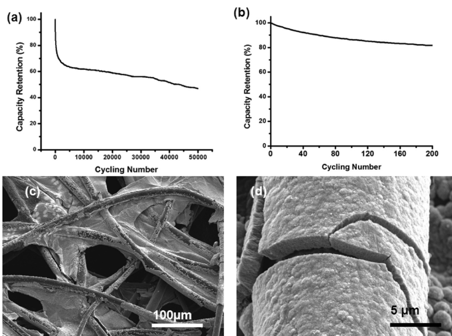
Figure 9. (a,b) Capacity retention of a full cell. (c,d) SEM images of \text{MnO}_2 -CNT-textile after 50 000 cycles.
